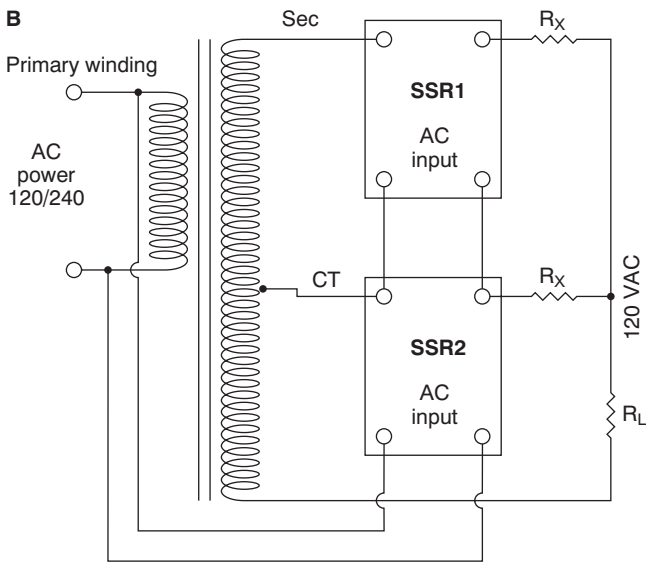
Fig. 20: Transformer tap switching
